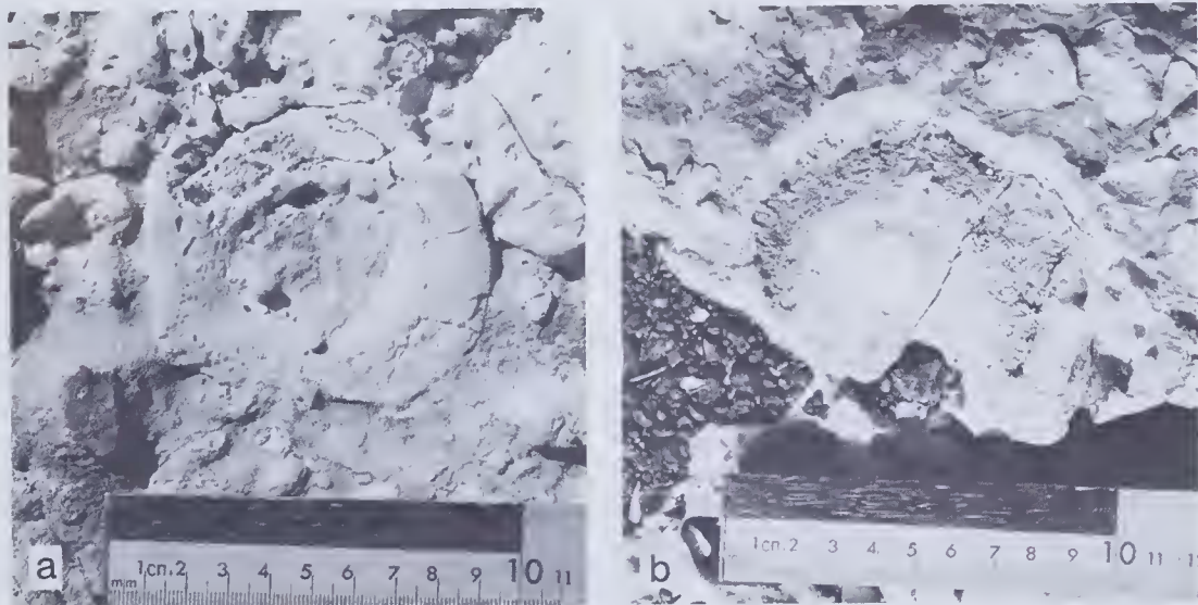
Fig. 8. Photographs of isolated adult ichthyosaur dorsal vertebral centra from Nightcliff: a, comparatively well preserved specimen consisting of silicified bone; b, a mould from which a specimen of dorsal vertebral centrum was recently removed by natural erosion or collector. The rib apophyses are well preserved.
